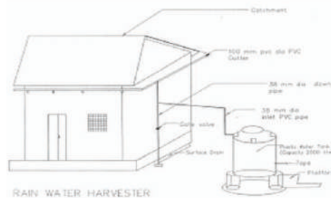
Figure 2 Rain Water Harvesting System: Source: DPHE
